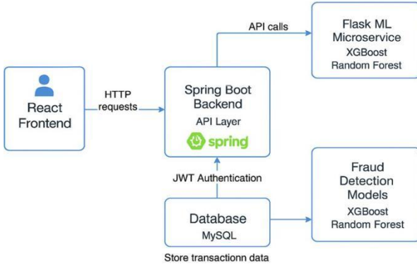
Fig. 1: System architecture of the hybrid fraud detection framework
