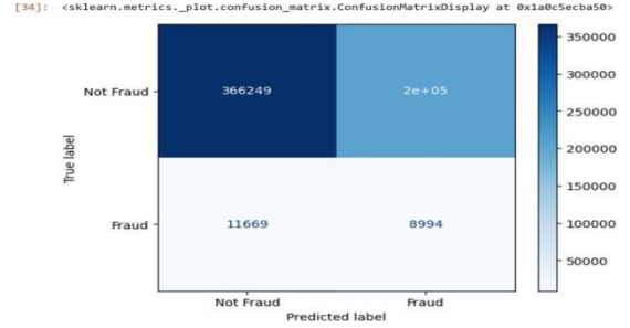
Fig. 4: Confusion matrix of classification results (showing false negatives).
